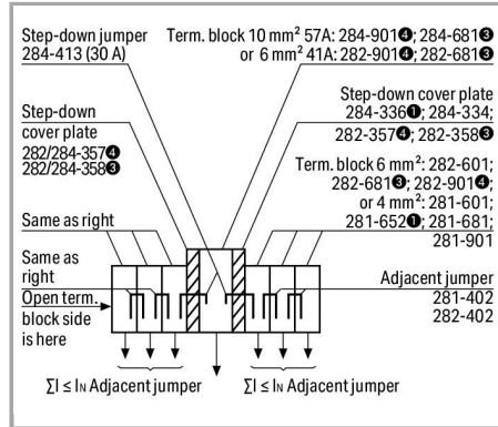
Assembly example: Commoning from 10 /6 mm 2 (8/10 AWG) to 6 mm 2 (10 AWG) rail-mount terminal blocks via step-down jumper (284-413).
