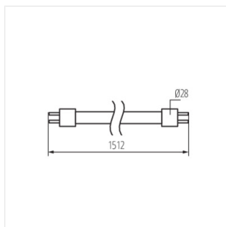
T8 LED GLASSv4 24W-CW
