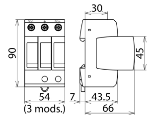
Dimension drawing DG M YPV SCI 1000
