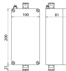
Dimension drawing ALGA 5
