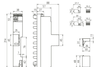
Dimension drawing DSH ZP 2 SG TT 255
