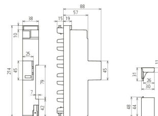
Dimension drawing DSH ZP 2 TT 255
