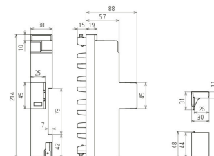
Dimension drawing DSH ZP 2 TNC 255
