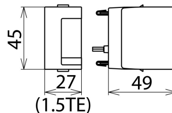
Dimension drawing DG MOD E DC 900
