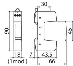
Dimension drawing DR M 2P 255 SN1802
