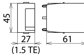
Dimension drawing DG MOD E H 1000 VA
