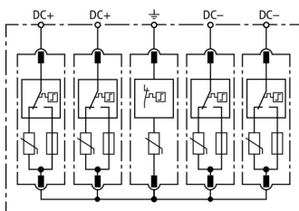
Basic circuit diagram DG M PV2 SCI 1000
