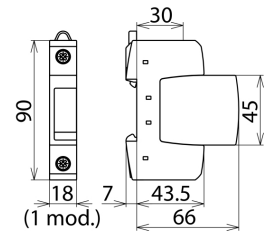
Dimension drawing DG S 275 VA
