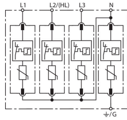
Basic circuit diagram DG MU 3PH 480 4W+G
