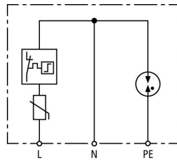
Basic circuit diagram DCOR L 2P 275
