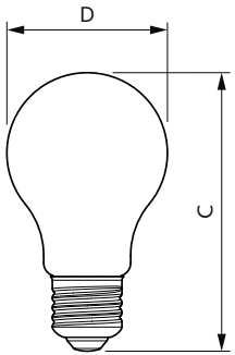
MAS LEDBulb DT7.2-75W E27 927A60CL G
