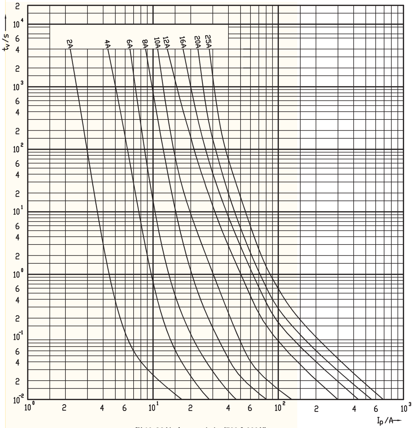
CH 10x38 I/t characteristics (700 & 900 V)
