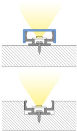
max. 14 mm
