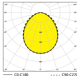
SALUKA-LED-PLUS/FROST-OP
