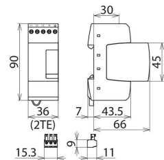
Dimension drawing DR M 4P 255 SN1872 FM
