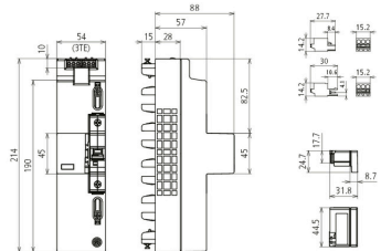
Dimension drawing DSH ZP 2 LSG A TT 255
