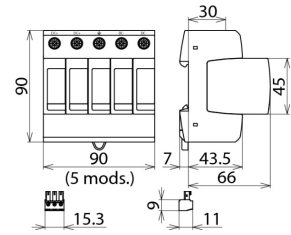
Dimension drawing DG M PV2 SCI 1000 FM
