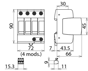
Dimension drawing DG M TNS 150 FM
