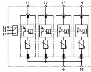
Basic circuit diagram DG M TNS 150 FM
