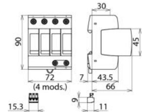
Dimension drawing DG M TT 150 FM
