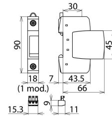
Dimension drawing DG S 48 FM
