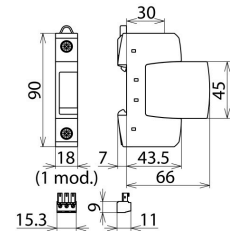
Dimension drawing DG S WE 600 FM
