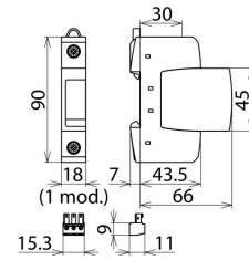
Dimension drawing DG S 600 FM
