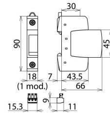
Dimension drawing DG S 275 VA FM
