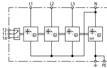
Basic circuit diagram DSH B TT 255 FM
