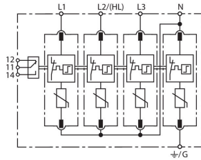
Basic circuit diagram DG MU 3PH 480 4W+G R
