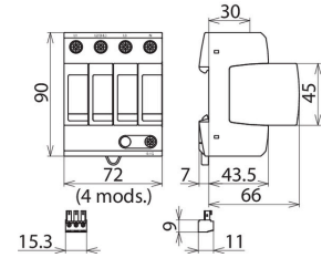
Dimension drawing DG MU 3PH 240 4W+G R
