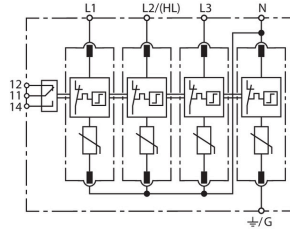
Basic circuit diagram DG MU 3PH 240 4W+G R
