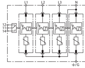
Basic circuit diagram DG MU 3PY 208 4W+G R
