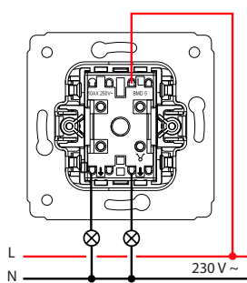
Double allumage
