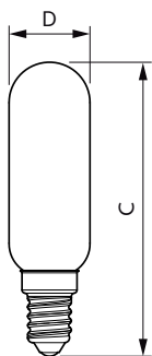
Bulb T25 230V 4.5-40W 470lm 2700K E14 CL
