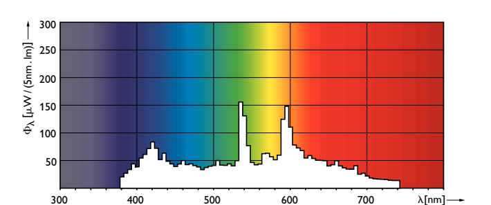
LDPO_CDM-T_35W_842-Spectral power distribution Colour
