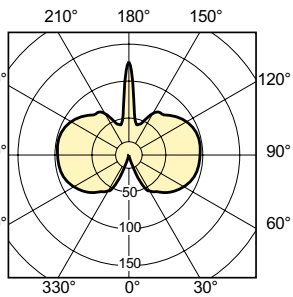
LDLD_CDM-T_0005-Light distribution diagram
