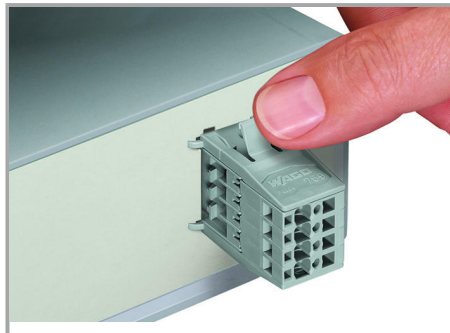
Male connector with snap-in flanges
