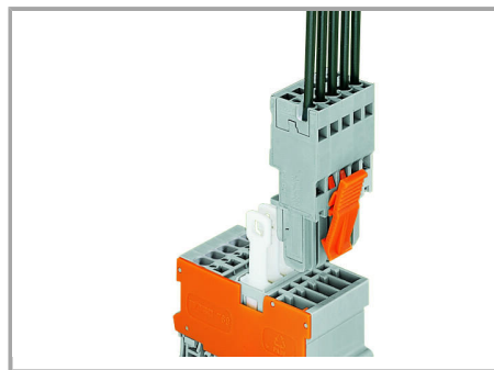
1-conductor/1-pin disconnect carrier terminal block
