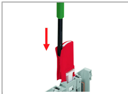
Unlocking a disconnect lock.
