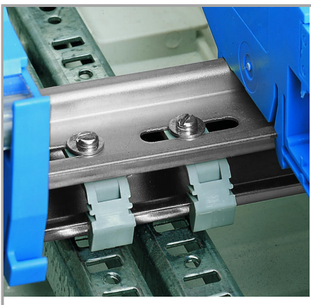
Isolated mounting of a carrier rail in a distribution box for protection class II
