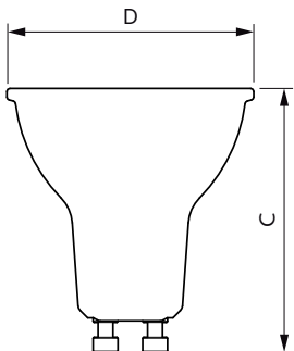
Corepro LEDspot 670lm GU10 830 60D
