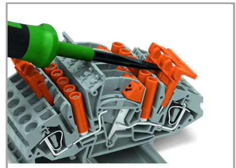
Jumper with safety lid:
