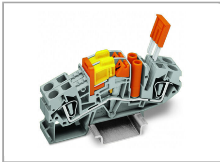
Transverse switching terminal blocks
