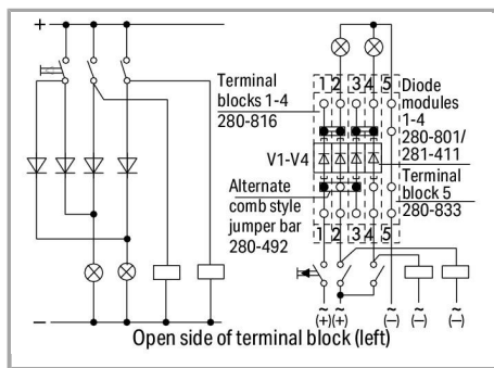
Lamp test circuit with blocking diodes
