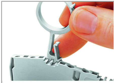
Clipping a wire harness support into the marker slot.
