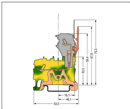
Ground carrier terminal block
