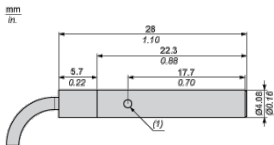
(1) LED
