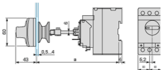
Door cut-out
