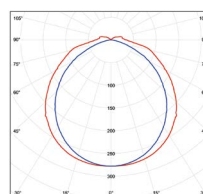
TRUST LED PS 2xT8/120CM
