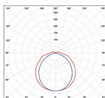
TRUST LED PS 2xT8/60CM
