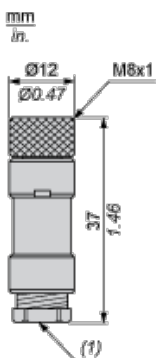
(1) Cable gland : M9.5 x 1
