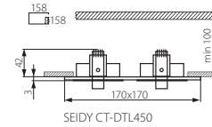
SEIDY CT-DTL450
