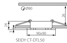
SEIDY CT-DTL50
