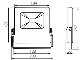
ANTOS LED 50W-NW B
